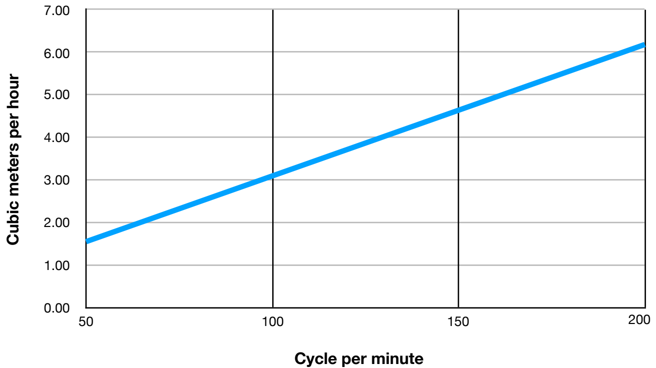
Displacement Flowrate in cubic meters per hour
